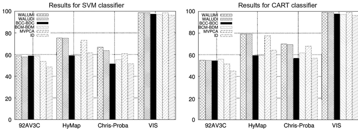
Fig. 4. SVM (polynomial) and CART classifier results for each image. Results cover until K = 15 .
