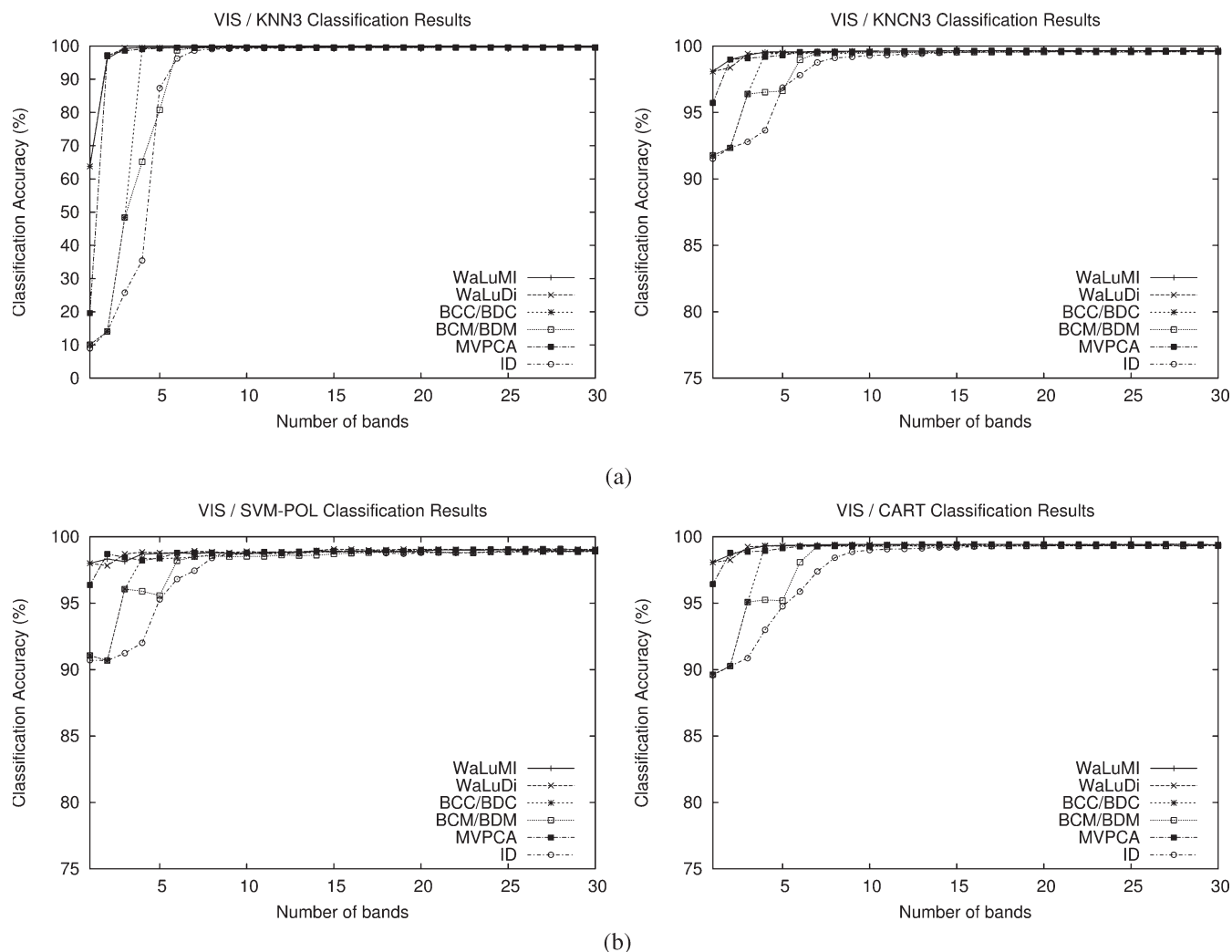
Fig. 7. (Top row) VIS DB–KNN3 and KNCN3, and (bottom row) SVM (polynomial) and CART classifiers.
