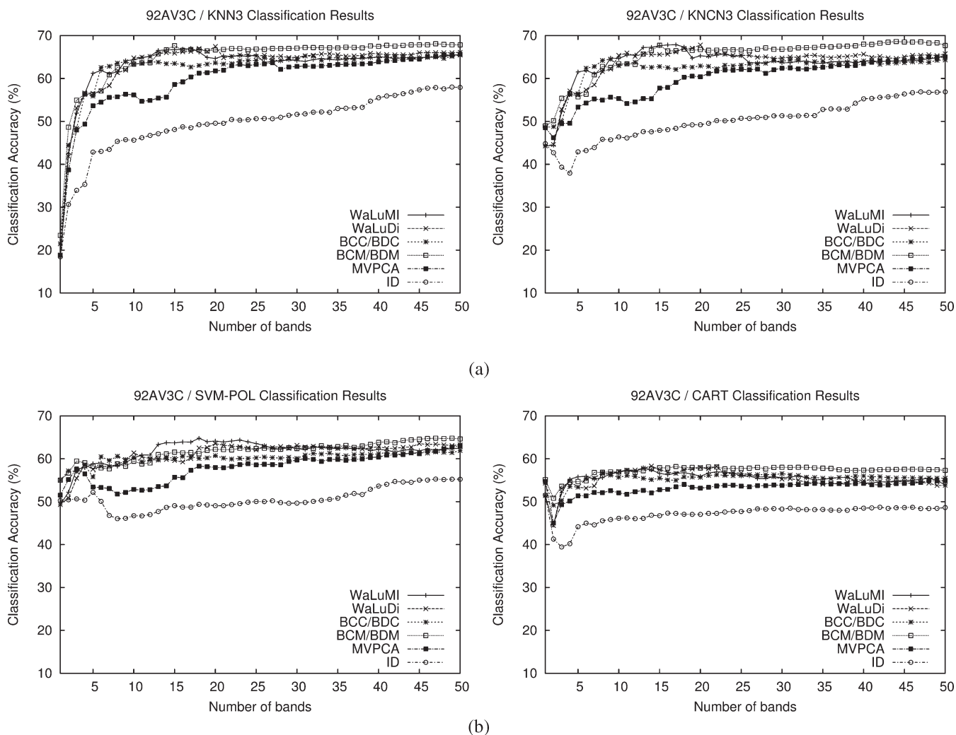
Fig. 5. (Top row) AV3C DB-KNN3 and KNCN3, and (bottom row) SVM (polynomial) and CART classifiers.
