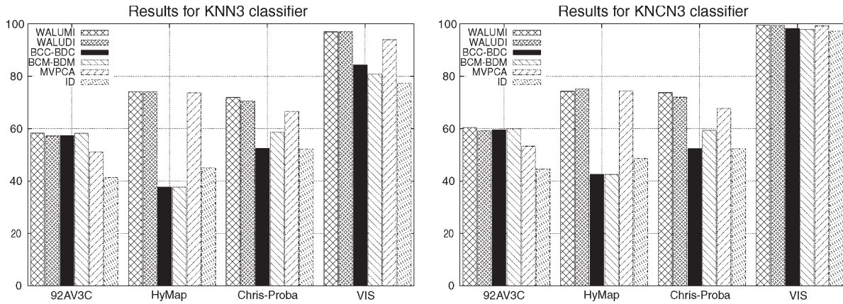
Fig. 3. KNN3 and KNCN3 classifier results for each image. Results cover the average classification rate up to K = 15 selected bands.
