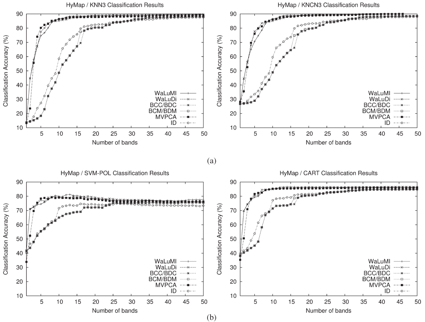
Fig. 6. (Top row) HyMap DB-KNN3 and KNCN3, and (bottom row) SVM (polynomial) and CART classifiers.
