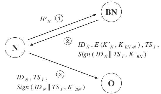
Figure 2. Node join in protocol 2
