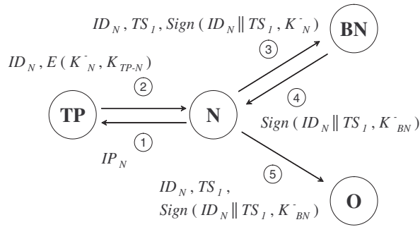
Figure 1. Node join in protocol 1
