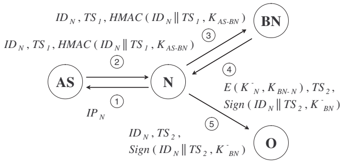
Figure 3. Node join in protocol 3
