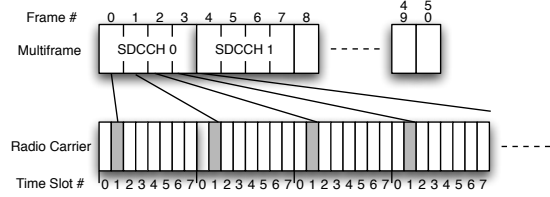
Figure 5: Timeslot 1 from each frame in a multiframe creates the logical SDCCH channel. In a single multiframe, up to eight users can receive SDCCH access.
